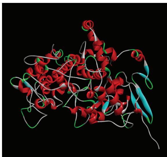
Validation of 6Y3C in BIOVIA.
