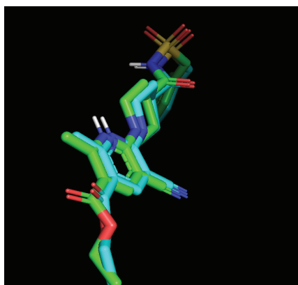
Validation of 4NTJ in PYMOL
