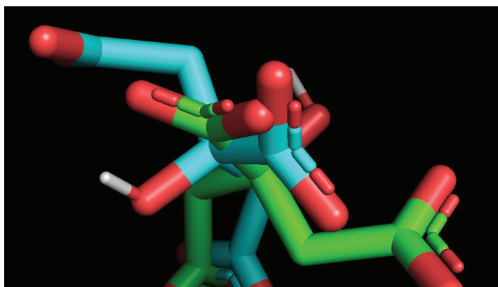
Validation of 6Y3C in PYMOL.
